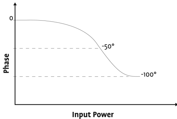
Figure 4 AM-PM Characteristic
